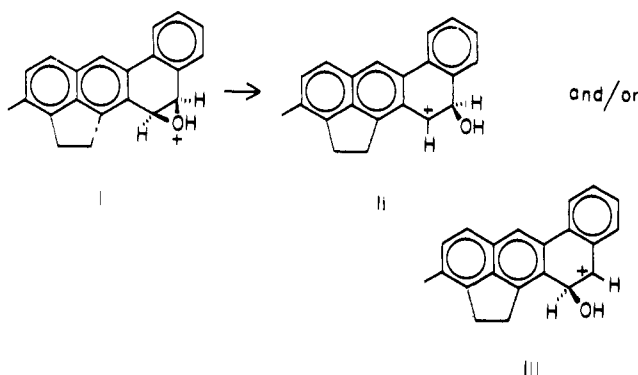
Figure 6. Two possible directions for the ring opening of protonated 3-methylcholanthrene oxide.
