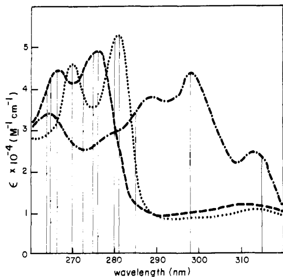
Figure 1. Uv spectra in 1:1 dioxane-water, 0.10 M in KCl, of various K-region derivatives of benz[ a ]anthracene: (.....) 5,6-oxide ( 2 ); (---) -5,6-dihydrodiol ( 6 ), (-·-·-) 5- + 6-hydroxy- ( 10 + 11 ). Regression analysis wavelengths are indicated by the vertical lines.
