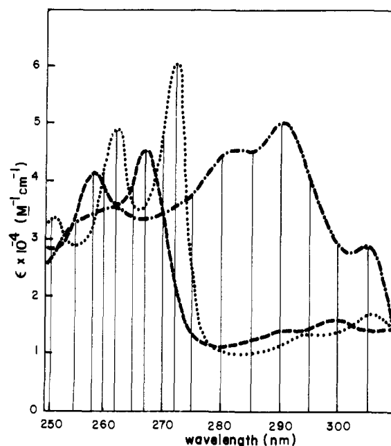
Figure 3. Uv spectra in 1:1 dioxane-water, 0.10 M in KCl, of various K-region derivatives of 3-methylcholanthrene: (.....) 11,12-oxide ( 4 ), (---) -11,12-dihydrodiol ( 8 ), (-·-·-) 11-hydroxy- ( 19 ). Regression analysis wavelengths are indicated by the vertical lines.
