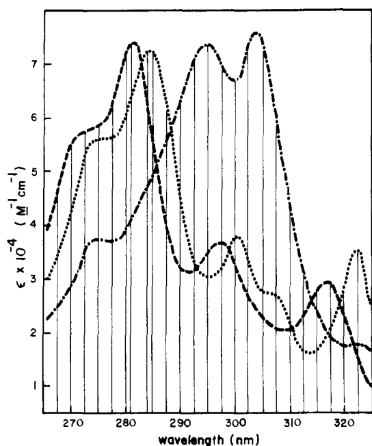
Figure 2. Uv spectra in 1:1 dioxane-water, 0.10 M in KCl, of various K-region derivatives of dibenz[ a,h ]anthracene: (.....) 5,6-oxide ( 3 ), (---) -5,6-dihydrodiol ( 7 ), (-·-·-) 5- + 6-hydroxy- ( 14 + 15 ). Regression analysis wavelengths are indicated by the vertical lines.
