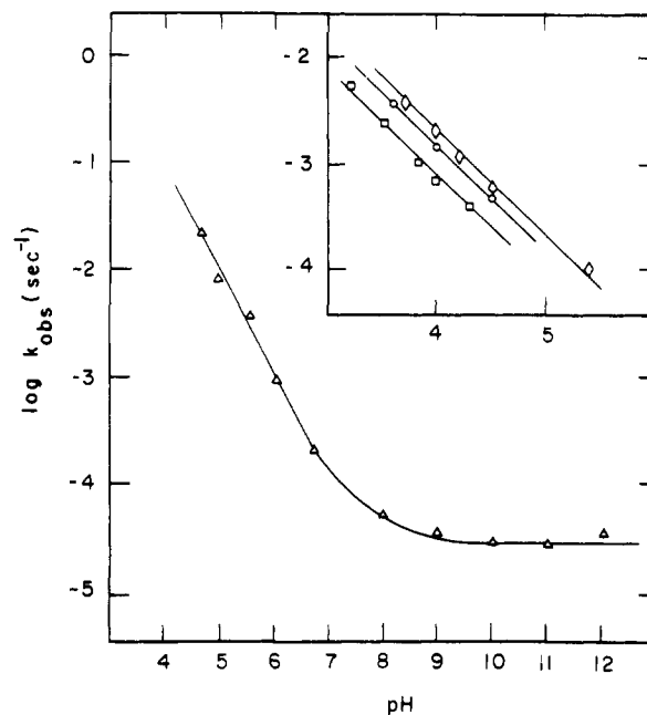
Figure 4. Plots of \log k_{\text{obsd}} (\text{s}^{-1}) vs. pH for solvolysis of various arene oxides in 1:1 dioxane-water, 0.10 M in KCl, at 36.8 °C: \square , 1 ; \circ , 2 ; \diamond , 3 ; \triangle , 4 .
