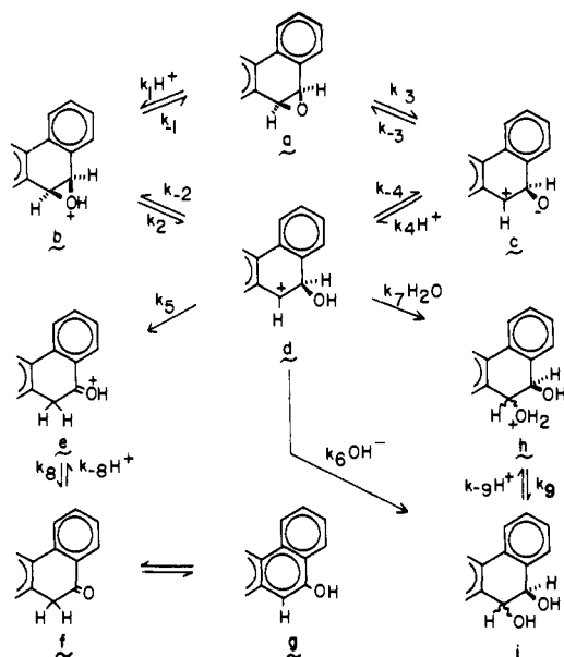
Figure 5. A mechanistic scheme that leads both to K-region phenols and K-region dihydrodiols from K-region oxide solvolysis. Only one of the two possible directions of ring opening is illustrated.
