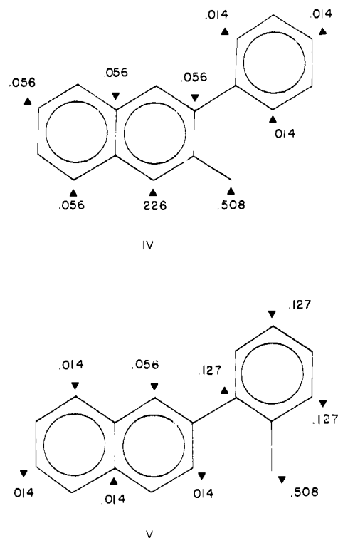
Figure 7. Hückel MO approximation of positive charge density in the two parent isomeric arylmethyl cations generated by scission of either the C 6 –O bond of protonated benz[ a ]anthracene oxide (IV) or C 5 –O bond (V). Triangles identify the charge-carrying atoms, which are labeled with the calculated fraction of charge residing at the carbon.
