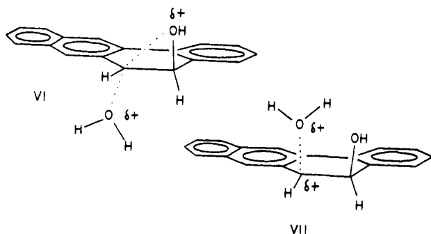
Figure 8. Possible transition states in formation of trans and cis dihydrodiols (VI and VII, respectively) from attack of water on a 5H-5-hydroxybenz[a]anthracen-6-yl cation.
