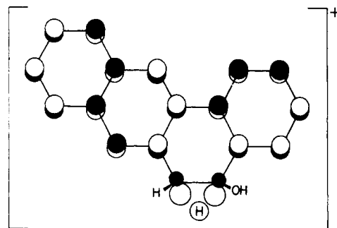
Figure 9. Transition state in the NIH rearrangement pathway of the 5H-5-hydroxybenz[a]anthracen-6-yl cation. Basis orbitals are shaded to represent HOMO of benz[a]anthracene 31 with a 1,6 (or 1,18) suprafacial hydrogen shift in progress.
